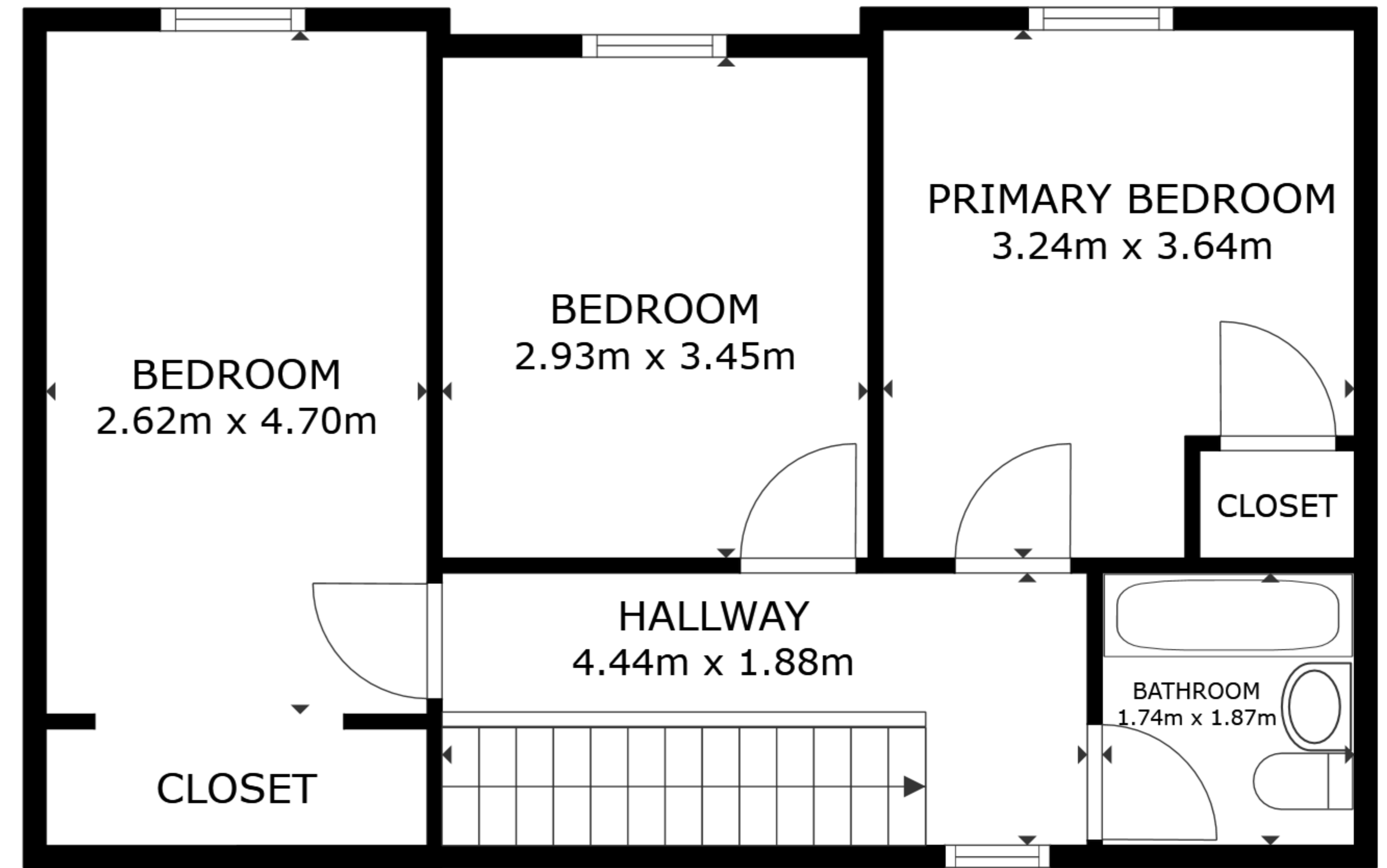
FLOOR 2
