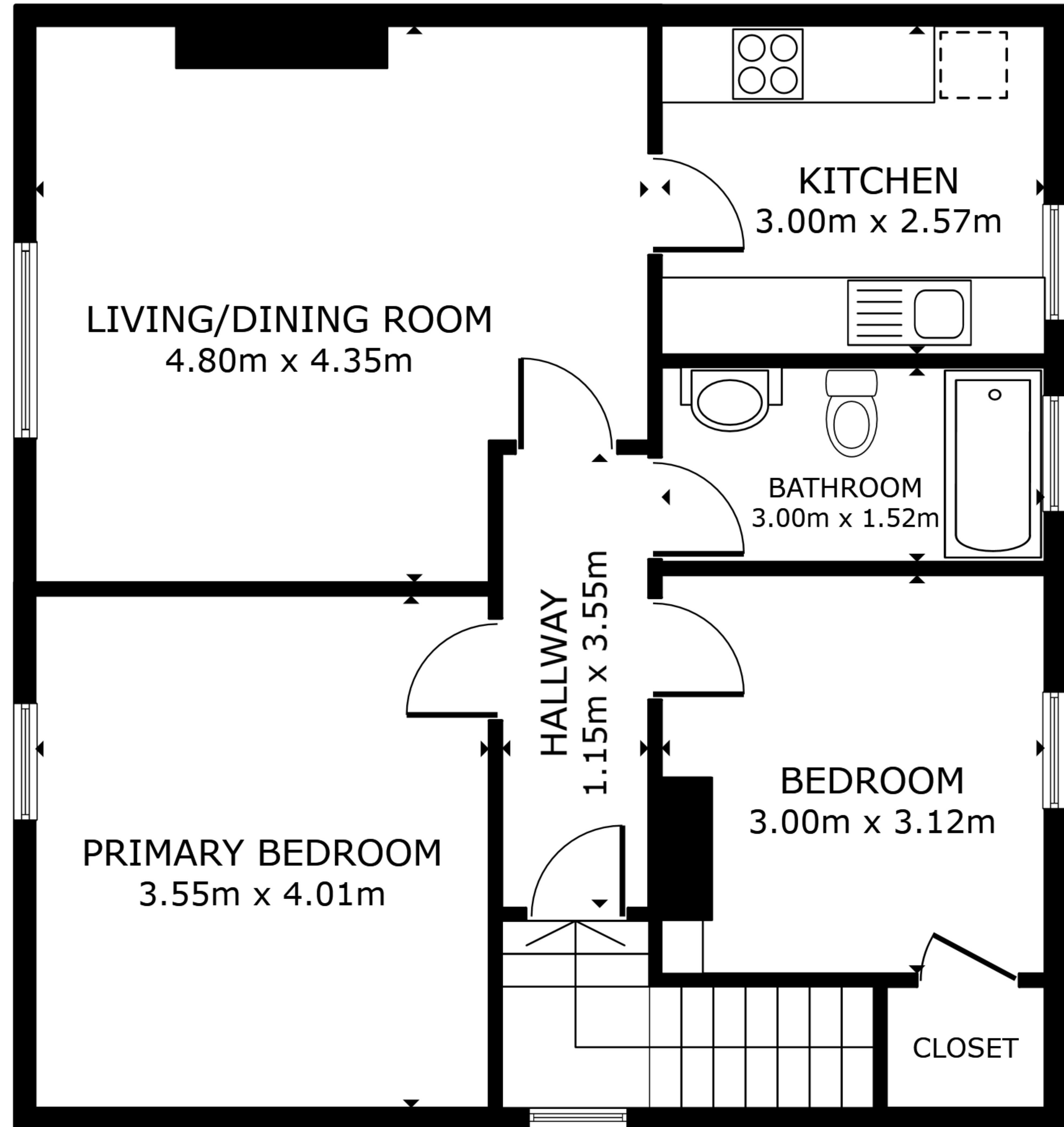
FLOOR 1
